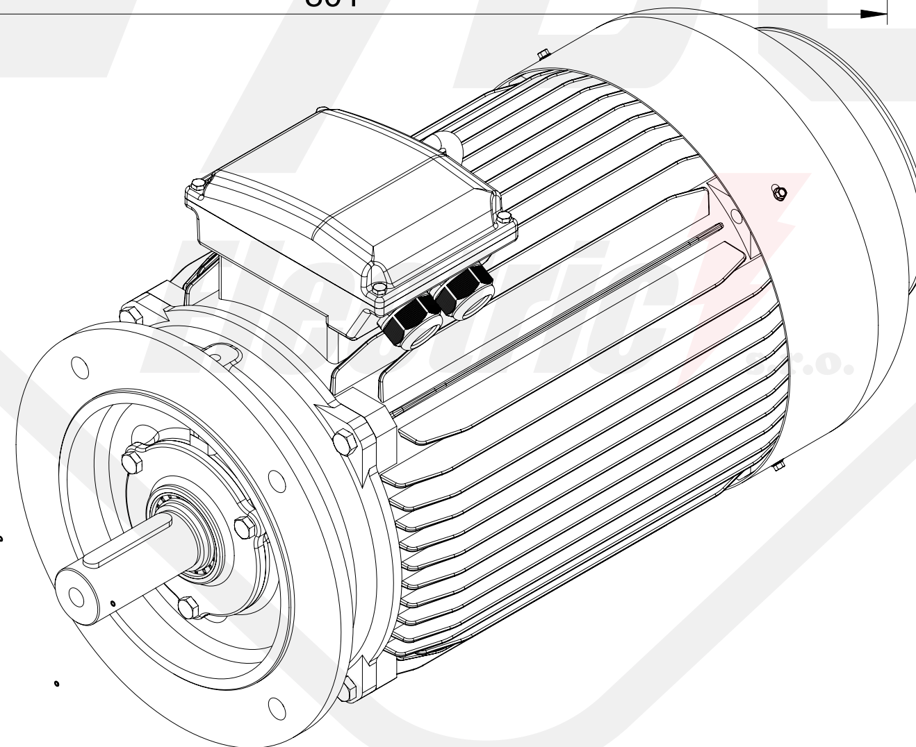
3LC-180L-B5 Mounting diagram
